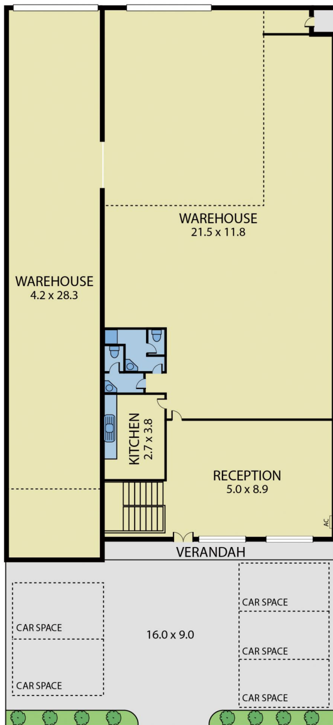
GROUND FLOOR
