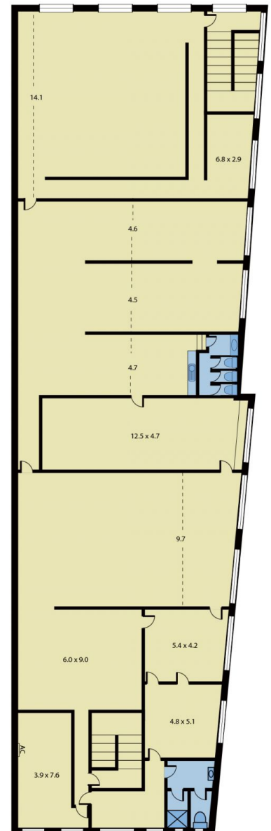
SECOND FLOOR
