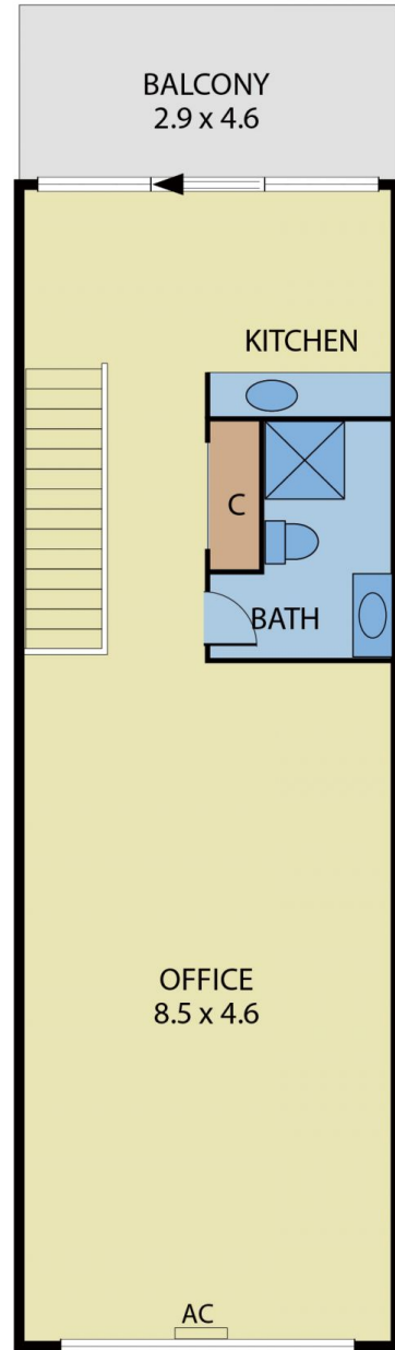
SECOND FLOOR
